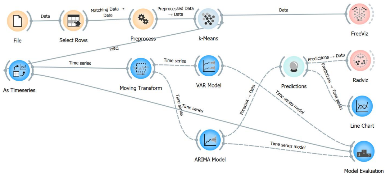
Figure 1: Proposed framework
