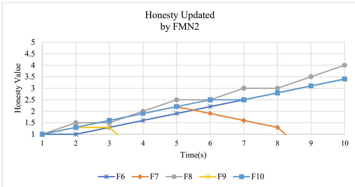
Figure 14: Honesty Updated by FMN2
