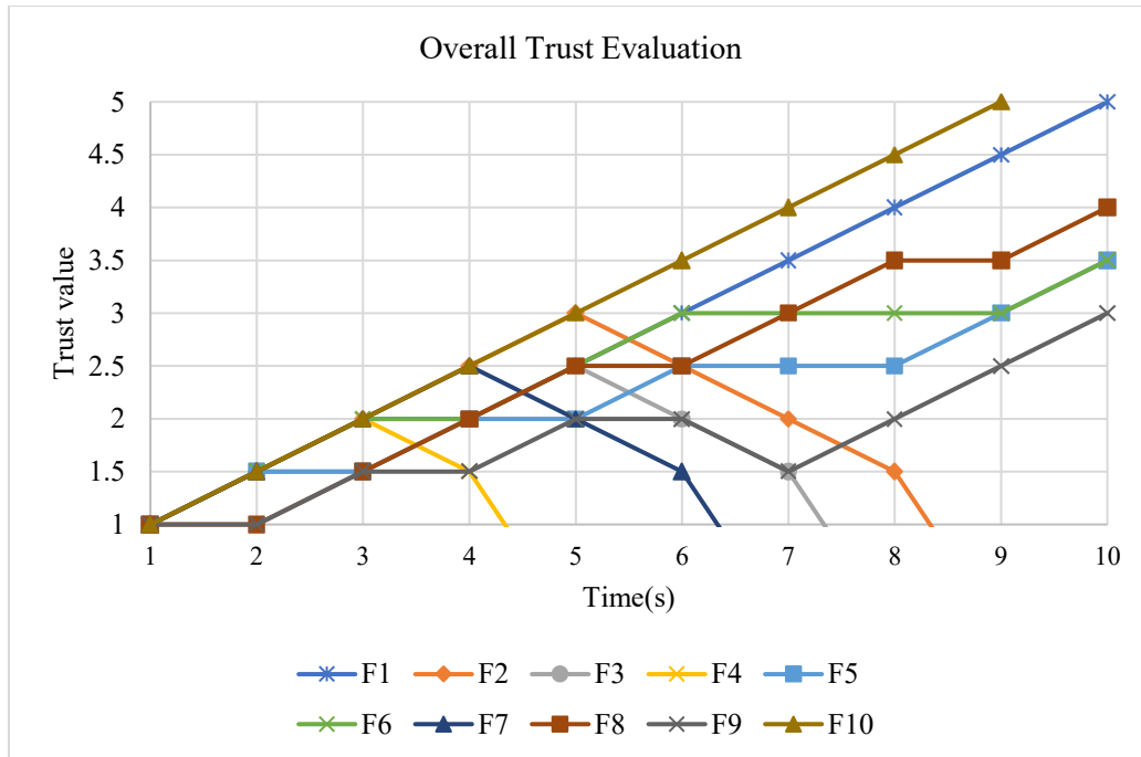
Figure 6: Trust Evaluation of all Fog nodes by their Fog Manager nodes (FMN)
