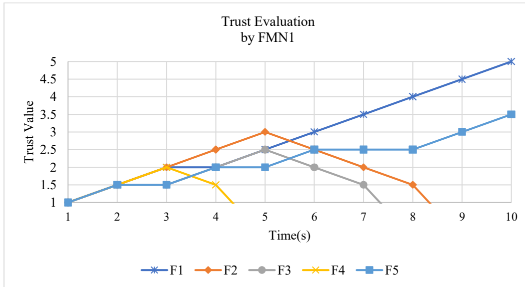
Figure 4: Trust Evaluation of Fog Nodes by Fog Manager Node (FMN1)
