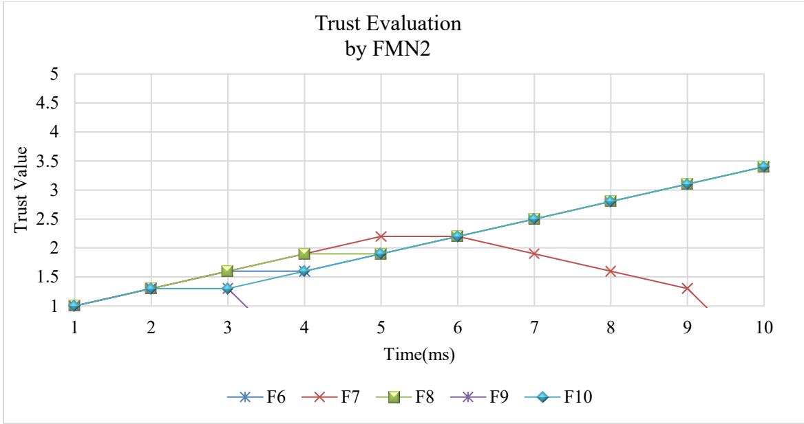
Figure 11: Trust Evaluation by FMN2
