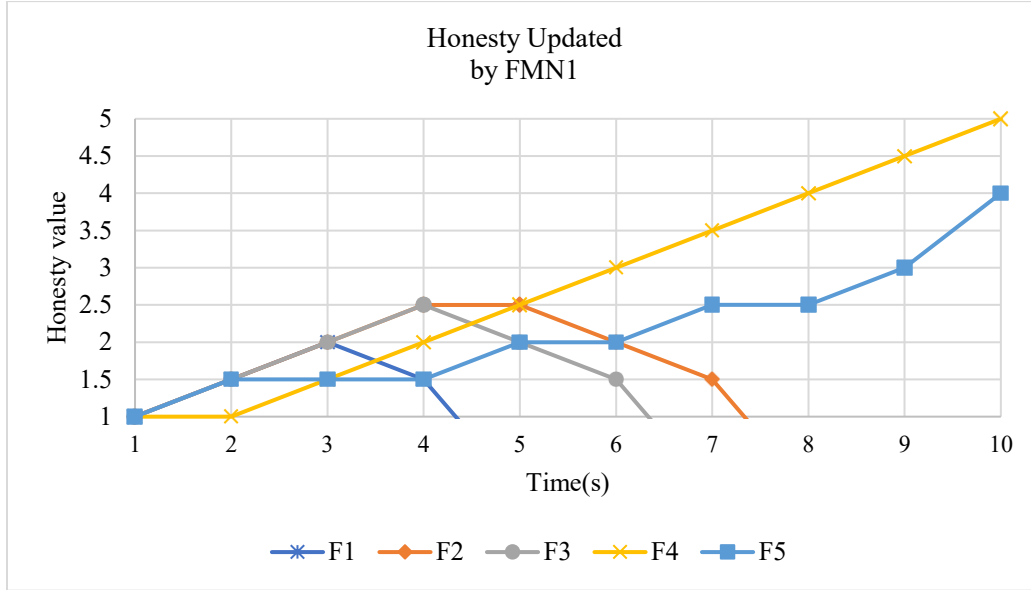
Figure 7: Honesty Updating of Fog Nodes by Fog Manager node (FMN1)
