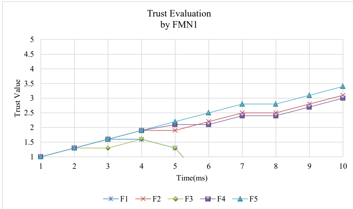
Figure 10: Trust Evaluation by FMN1
