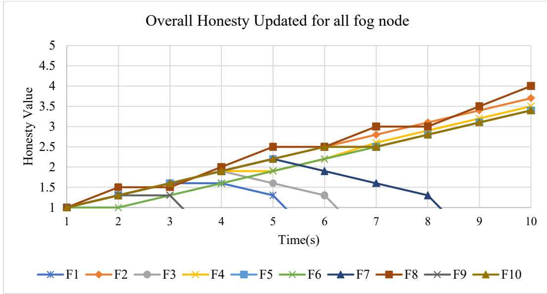
Figure 15: Overall Honesty Updated for all Fog Nodes
