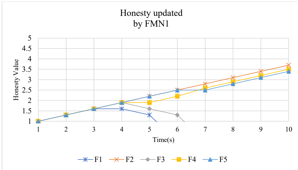
Figure 13: Honesty Updated by FMN1
