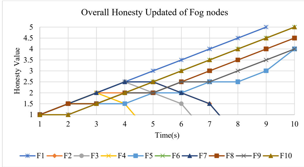
Figure 9: Honesty Updating of all Fog Nodes by their Fog Manager Nodes (FMN)
