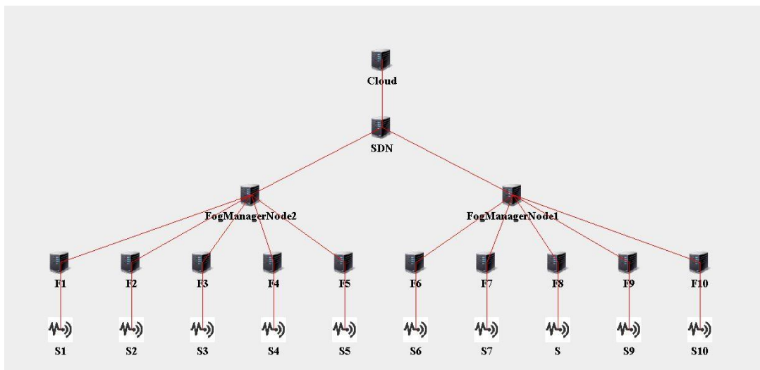
Figure 3 Overall Simulated Architecture in iFogSim
