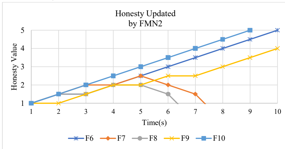
Figure 8: Honesty updating of Fog Nodes by Fog Manager Node (FMN2)
