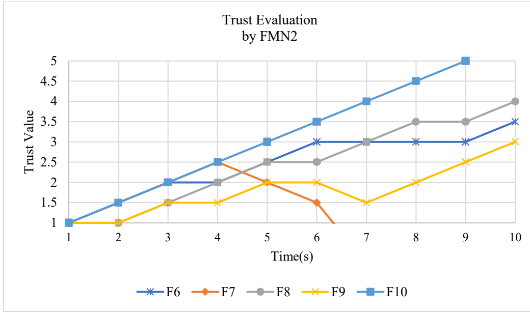
Figure 5: Trust Evaluation of Fog nodes by Fog Manager Node (FMN2)
