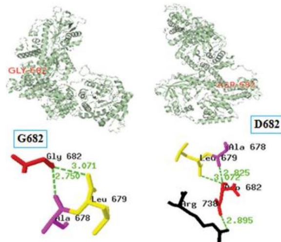
Figure 11: rs113914406 (G682D)
