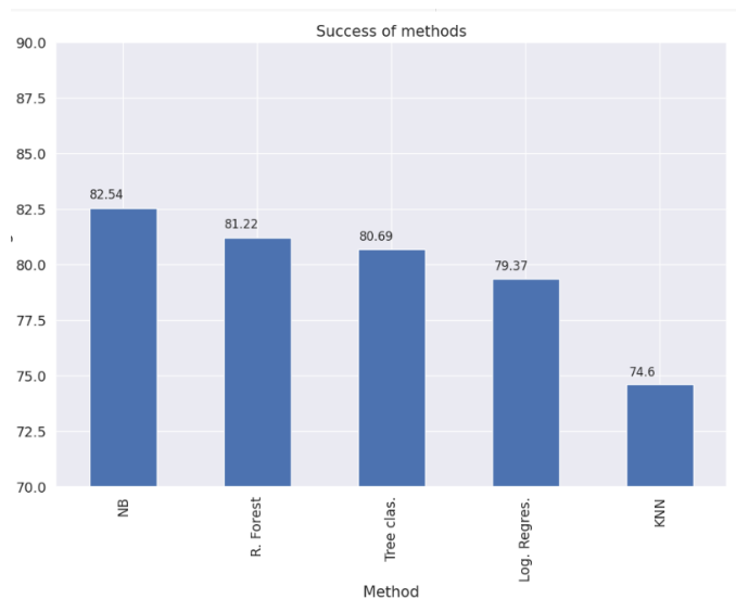
Figure 34: Classification Accuracy Results of ML Classifiers
