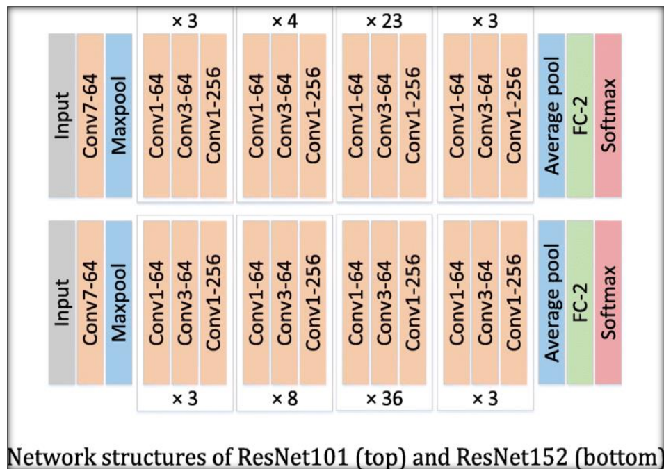
Figure 5: ResNet101 Architecture
