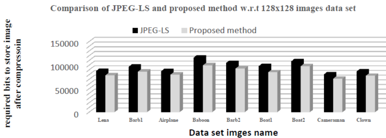
Figure 7: Comparison of JPEG-LS and proposed method w.r.t 128x128 images data set
