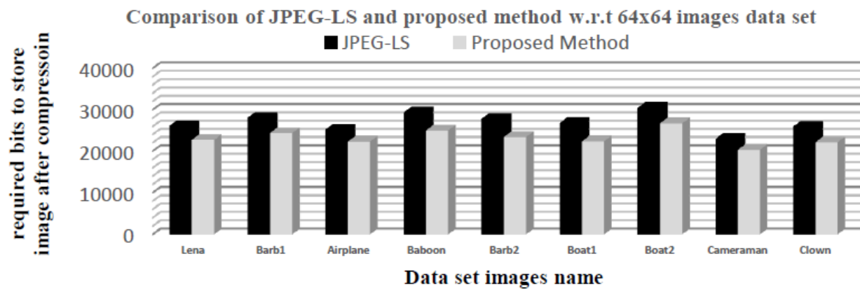
Figure 6: Comparison of JPEG-LS and proposed method w.r.t 64x64 images data set
