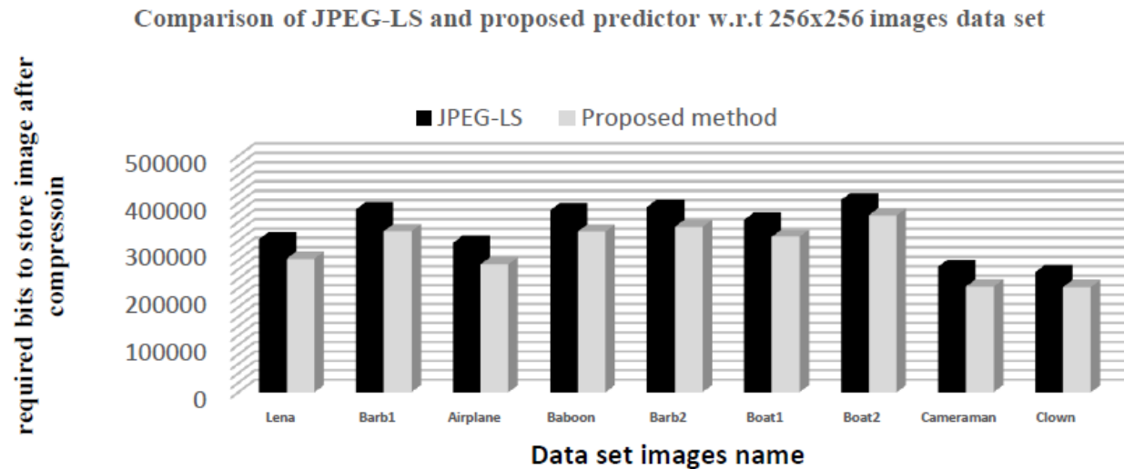
Figure 8: Comparison of JPEG-LS and proposed method w.r.t 256x256 images data set
