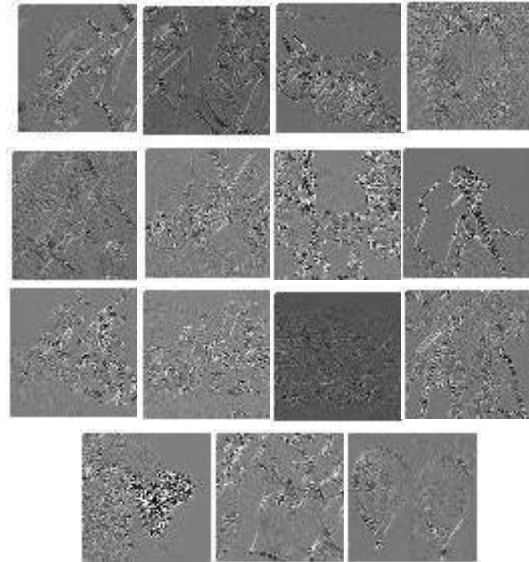
Figure 4: Prediction error after JPEG-LS predictor implementation
