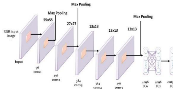
Figure 9: Detailed Architecture of Alexnet
