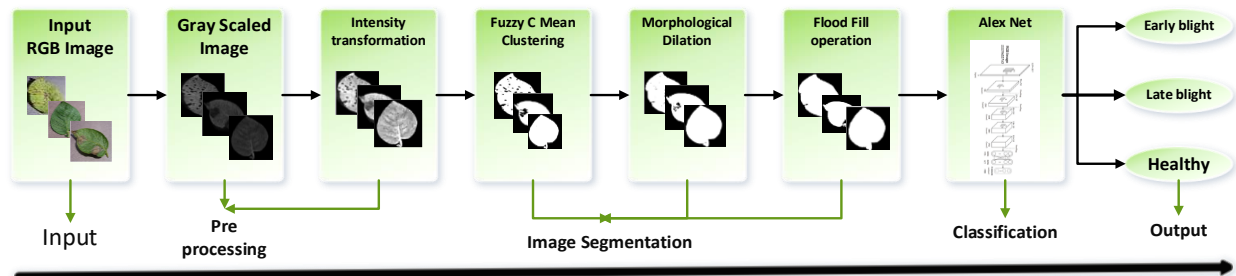
Figure 1: Block diagram of the proposed method for the disease detection of potato leaves
