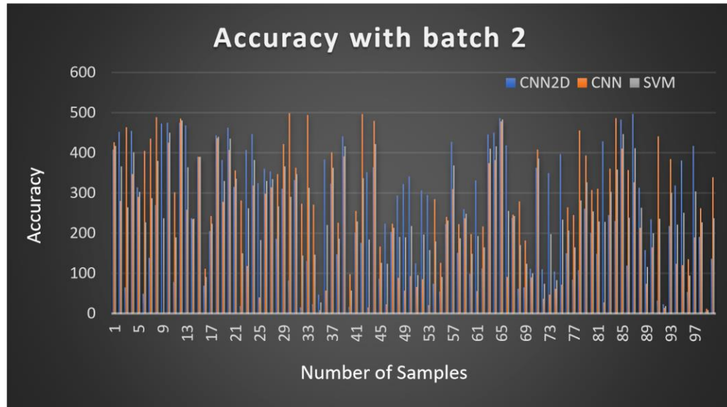
Figure 5: Accuracy results with batch 2
