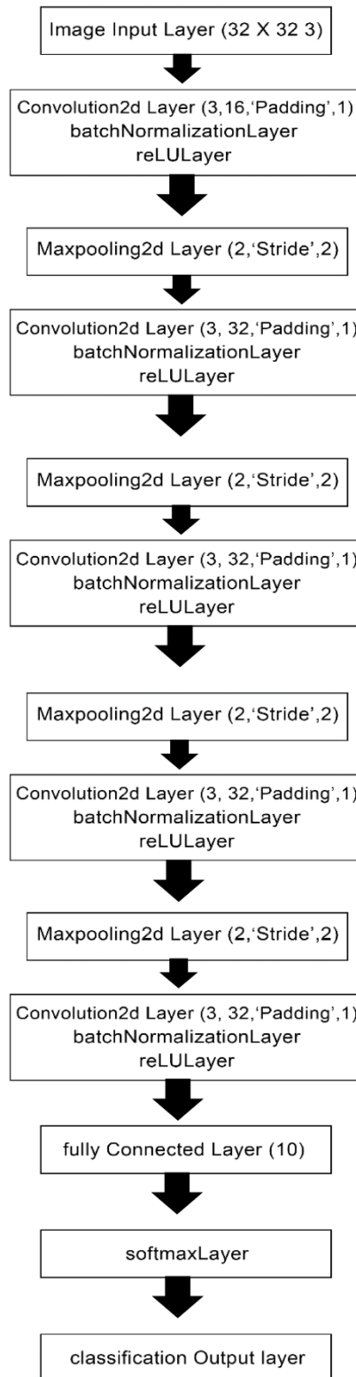
Figure 3: Proposed 2D CNN Model Layered Architecture
