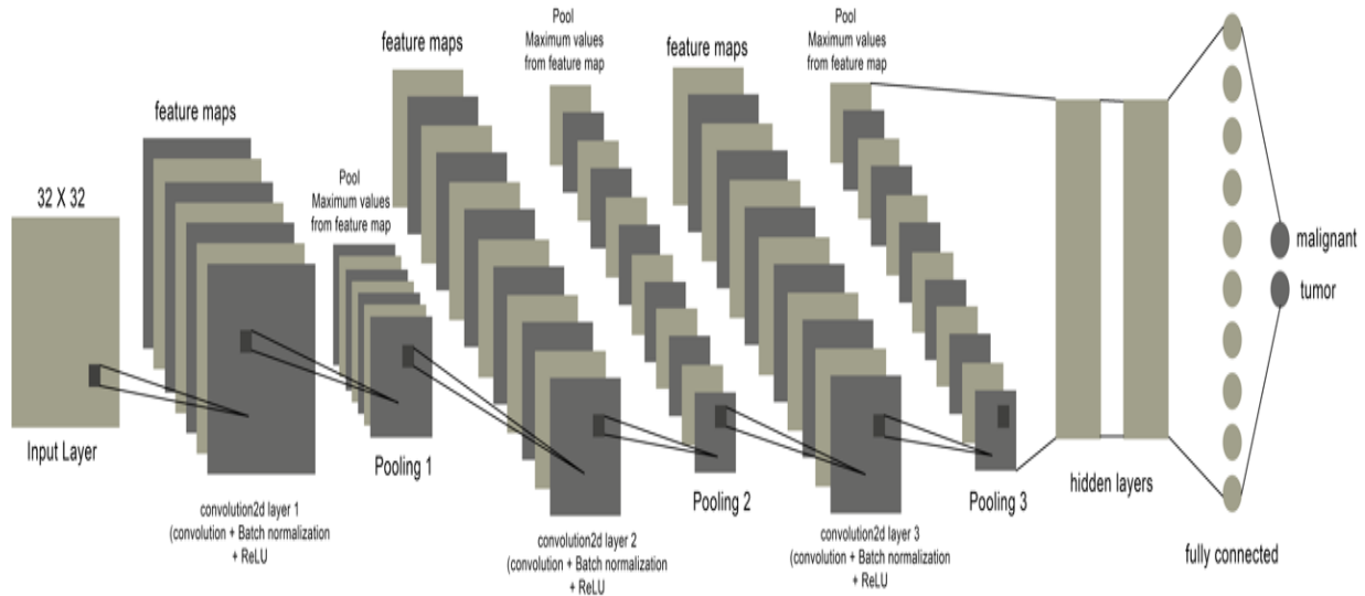
Figure 2: The architectural structure of the CNN process
