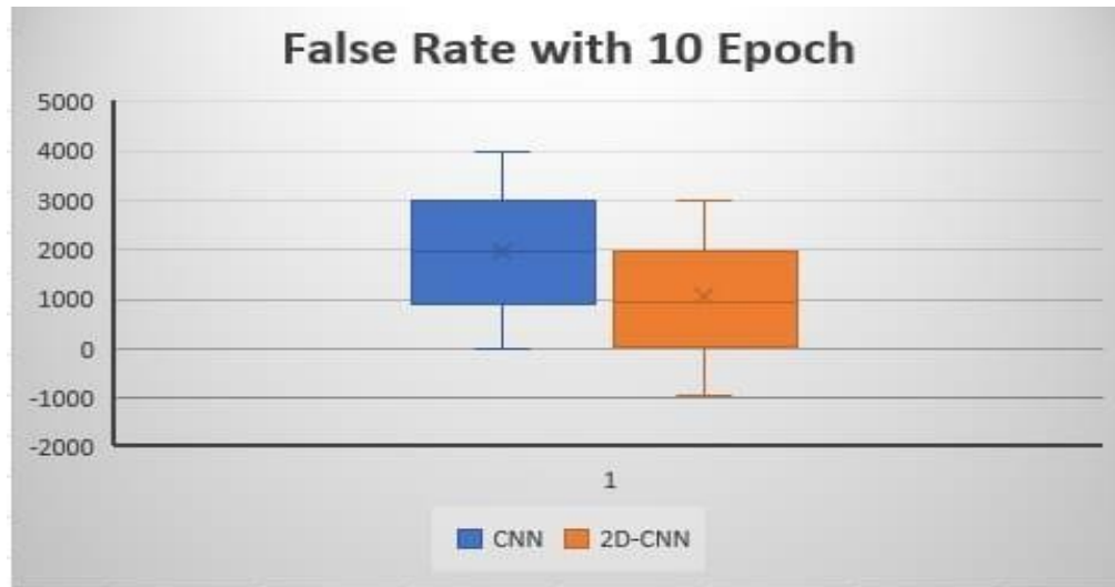
Figure 9: False results of epoch 10 with batch 3
