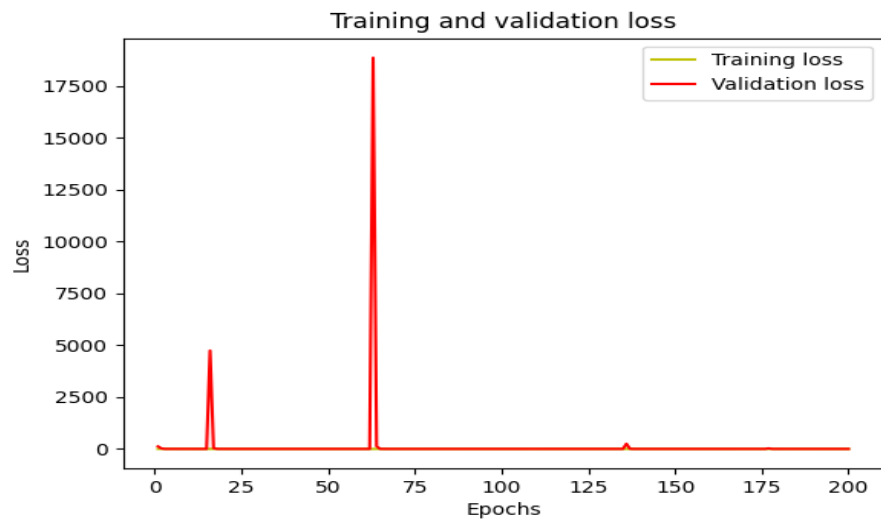
Figure 5: Training and Validation Losses on BZNet
