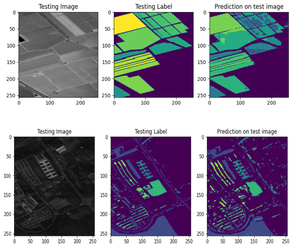
Figure 6: Predictions of Two Test Images on proposed model
