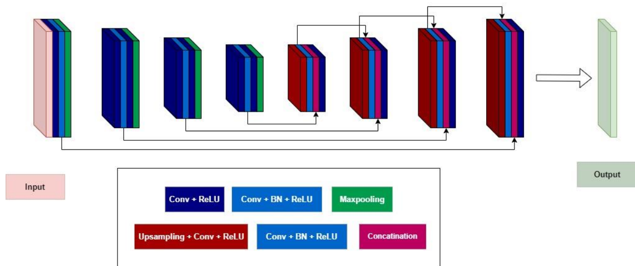
Figure 1: BZNet Architecture
