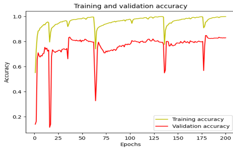
Figure 4: Training and Validation Accuracy of BZNet
