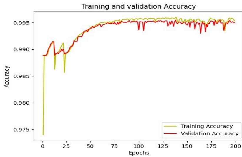
Figure 3: Accuracy of Training and Validation UNET
