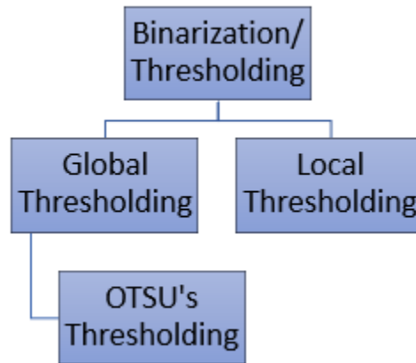
Figure 6: Binarization Techniques
