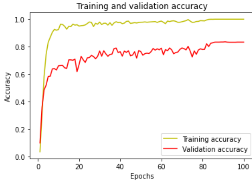
Figure 11: Training and Validation Accuracy on Custom dataset
