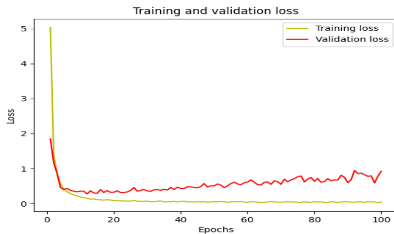
Figure 8: Training and Validation Loss on UHAT dataset
