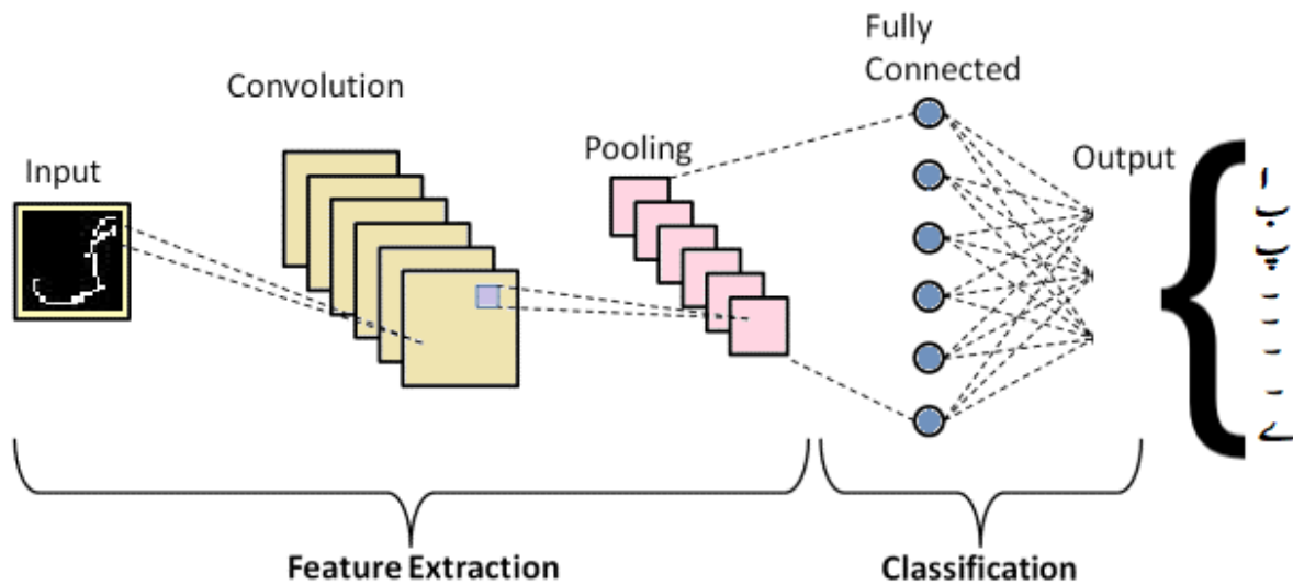
Figure 7: Proposed Architecture
