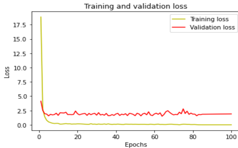
Figure 9: Training and Validation Loss on Custom dataset
