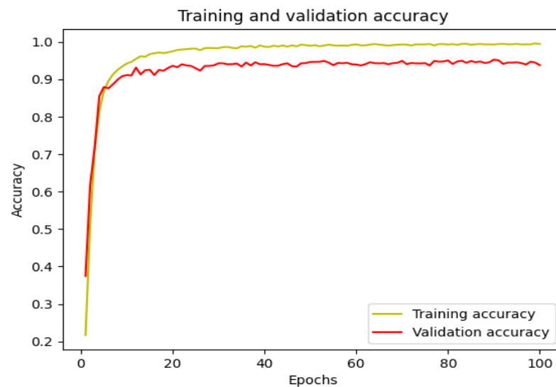
Figure 10: Validation and Training Accuracy on UHAT dataset
